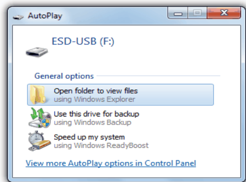
Figure 5.1. AutoPlay Box
